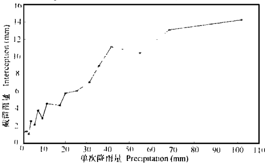
图 1 甜槠林林冠截留雨量与降水量之间的关系 Fig. 1 Relationship between precipitation and canopy interception in C. eyrei forest
