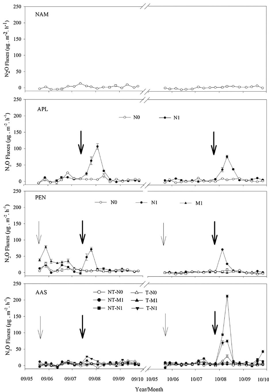
Fig. 2. Daily N 2 O emissions from different land uses as affected by different management practices during the study period. NAM: native alpine meadow with winter grazing; APL: abandoned pasture; PEN: perennial Elymus nutans Griseb. pasture; AAS: annual Avena sativa L. pasture. Arrows show fertilizer application dates. The thick arrow indicates sheep manure application and the thinner arrow indicates urea application. Bars indicate mean ± 1SE (n = 3).
