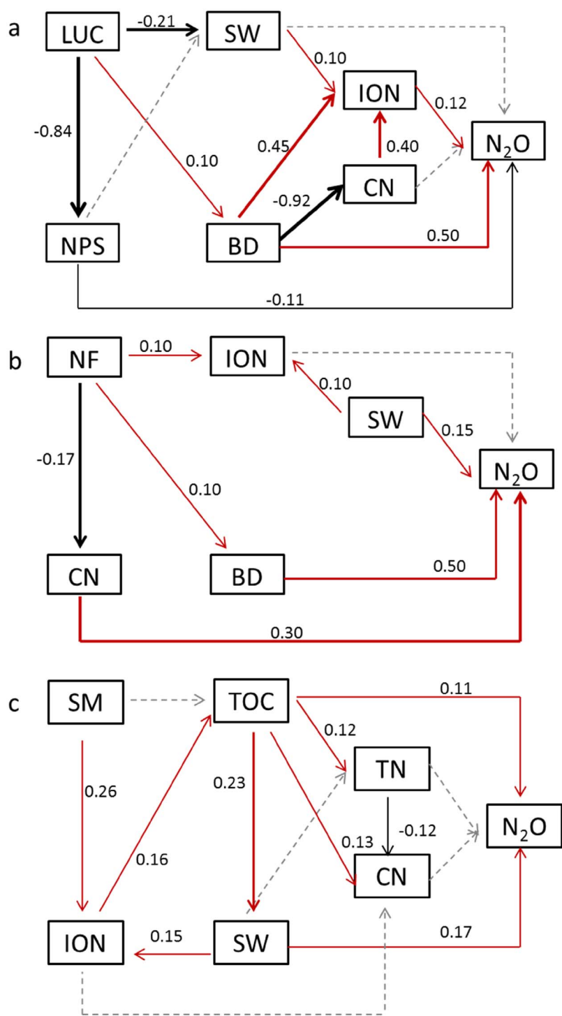
Fig. 5. The final SEM for cumulative N 2 O emissions affected by land use change (a, Fisher C = 3.99, p = 0.99, AIC = 55.99), N fertilizer addition (b, Fisher C = 5.1, p = 0.75, AIC = 33.1) and sheep manure addition (c, Fisher C = 4.17, p = 0.94, AIC = 60.17). Width of arrows indicates the strength of the relationships. Solid red arrows represent positive paths (p < 0.05), solid black arrows represent negative paths (p < 0.05) and dotted gray arrows represent non-significant paths (p > 0.05). LUC, land use change; SW, soil water content; BD, bulk density; TOC, soil total organic carbon; TN, soil total nitrogen, CN, soil C/N ratio; ION, soil inorganic N; NPS, number of plant species; NF, N fertilizer; SM, sheep manure. (For interpretation of the references to color in this figure legend, the reader is referred to the web version of this article.)
