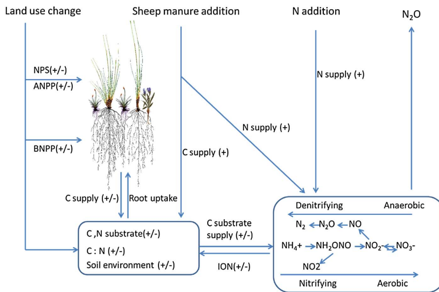
Fig 1. A conceptual model of how land use change and management practices regulate N_2O production and consumption processes (Liu and Greaver, 2009). NPS: the number of plant species; ANPP: aboveground net primary productivity; BNPP: belowground net primary productivity; C:N, soil C/N ratio; ION, soil inorganic N.
