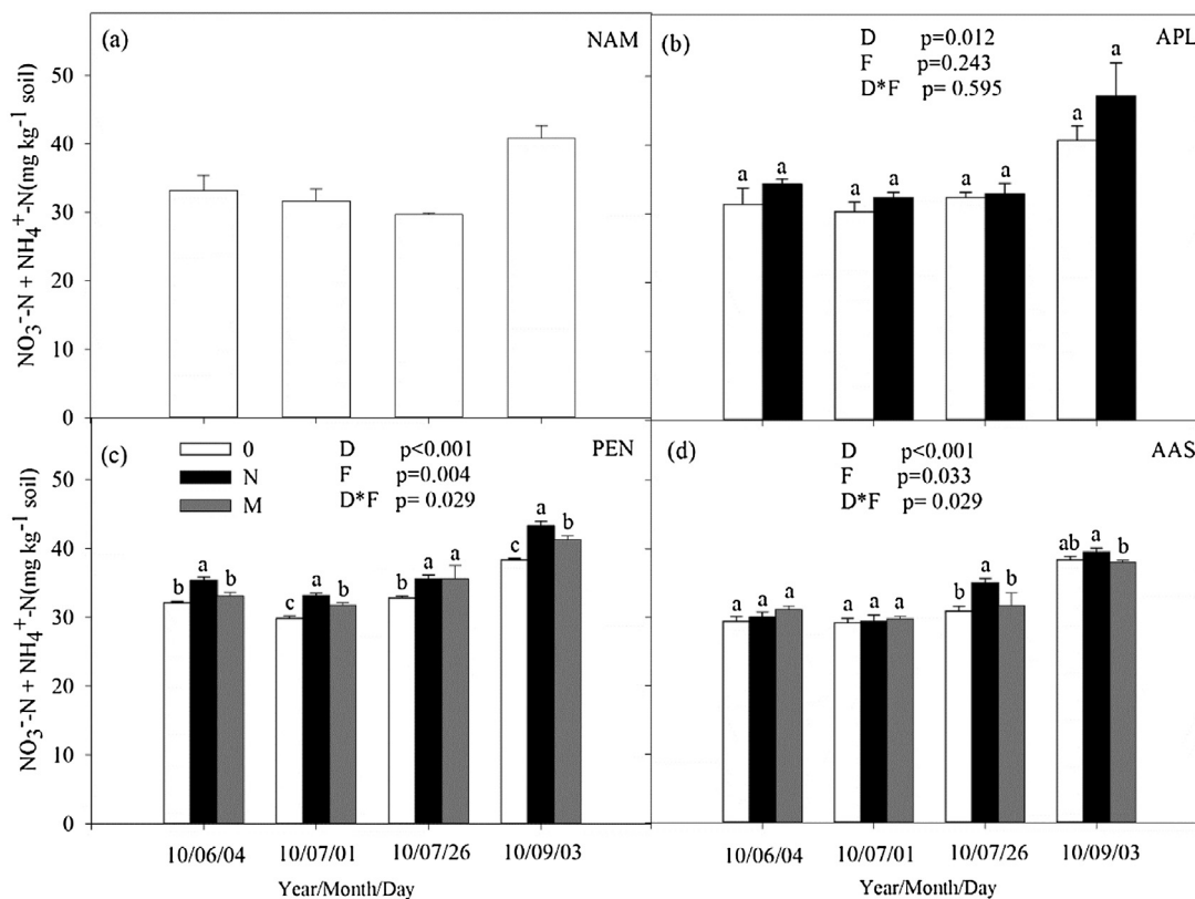
Fig. 3. (a): Seasonal variability of inorganic N ( \text{NO}_3^- \text{-N} + \text{NH}_4^+ \text{-N} ( \text{mg kg}^{-1} soil)) at a depth of 10 cm in NAM; (b): Seasonal variability of inorganic N ( \text{NO}_3^- \text{-N} + \text{NH}_4^+ \text{-N} ( \text{mg kg}^{-1} soil)) at a depth of 10 cm in APL with different managements; (c): Seasonal variability of inorganic N ( \text{NO}_3^- \text{-N} + \text{NH}_4^+ \text{-N} ( \text{mg kg}^{-1} soil)) at a depth of 10 cm in PEN with different management; (d): Seasonal variability of inorganic N ( \text{NO}_3^- \text{-N} + \text{NH}_4^+ \text{-N} ( \text{mg kg}^{-1} soil)) at a depth of 10 cm in AAS under different management. NAM: native alpine meadow with winter grazing; APL: abandoned pastureland; PEN: perennial Elymus nutans Griseb. pasture; AAS: annual Avena sativa L. pasture; D: sampling date; F: Fertilization; 0: without fertilizer; M: with sheep manure; N: with urea. Bars indicate mean \pm 1SE. Different letters above bars indicate significant differences among treatments at the p < 0.05 level.
